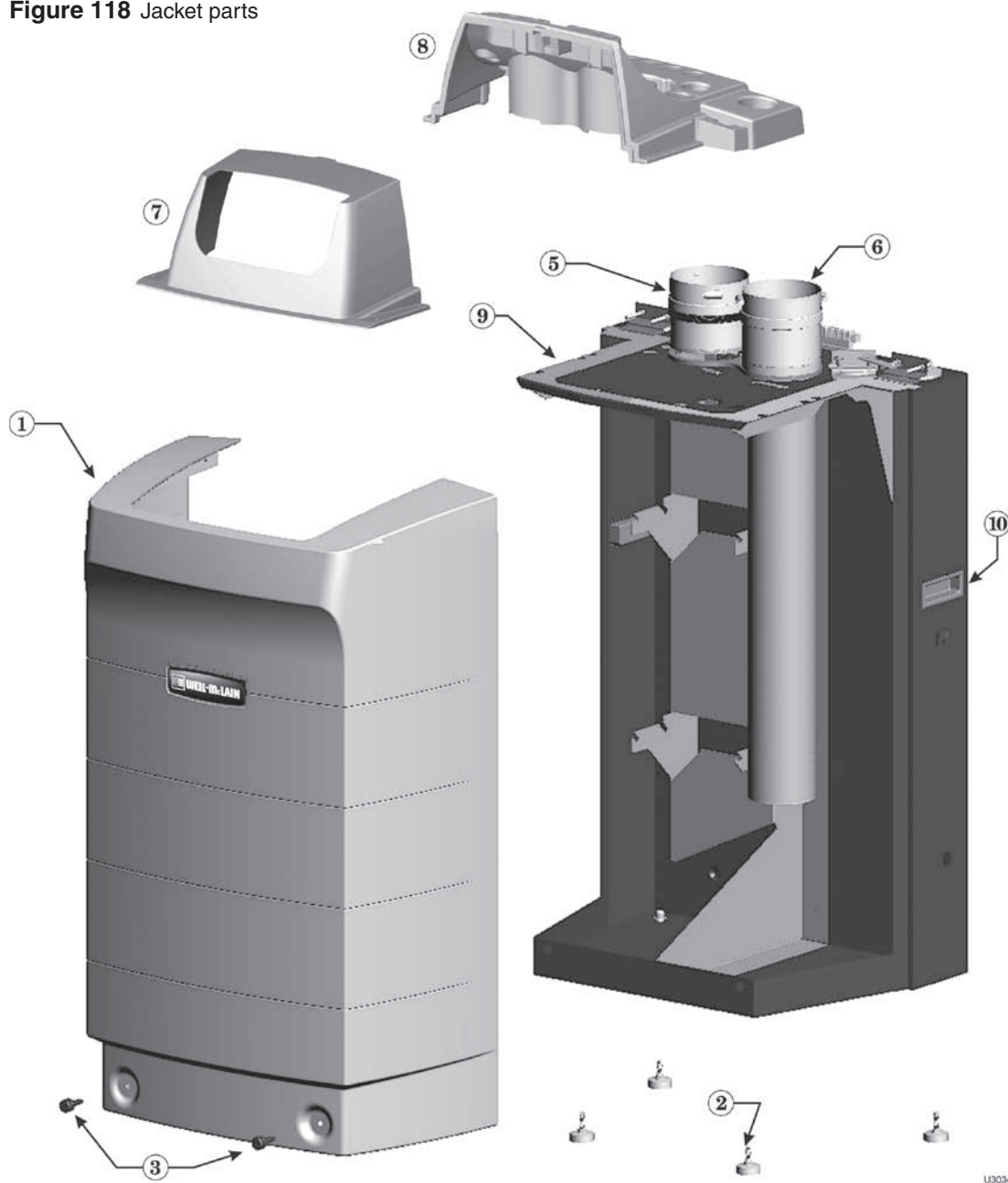
Figure 118 Jacket parts
